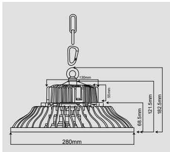
DIMENSIONS - 100W
