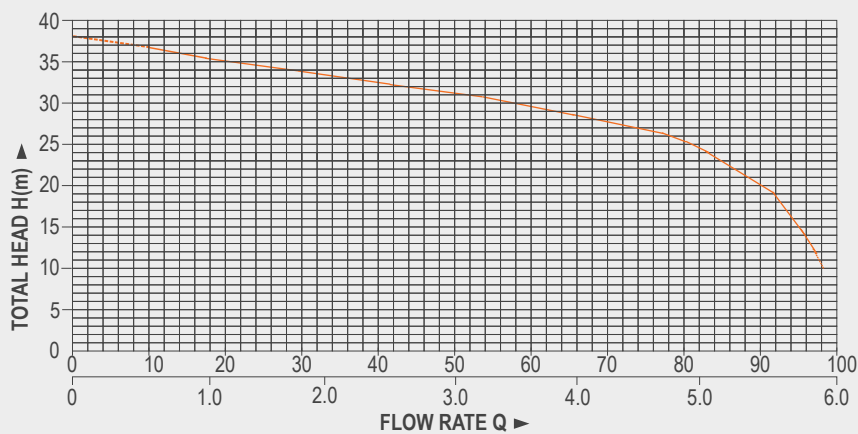
PERFORMANCE CHART AT n=2900rpm
