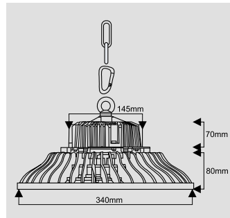
DIMENSIONS - 150W
