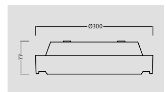
DIMENSIONS - 16W
