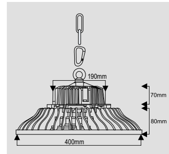
DIMENSIONS - 200W
